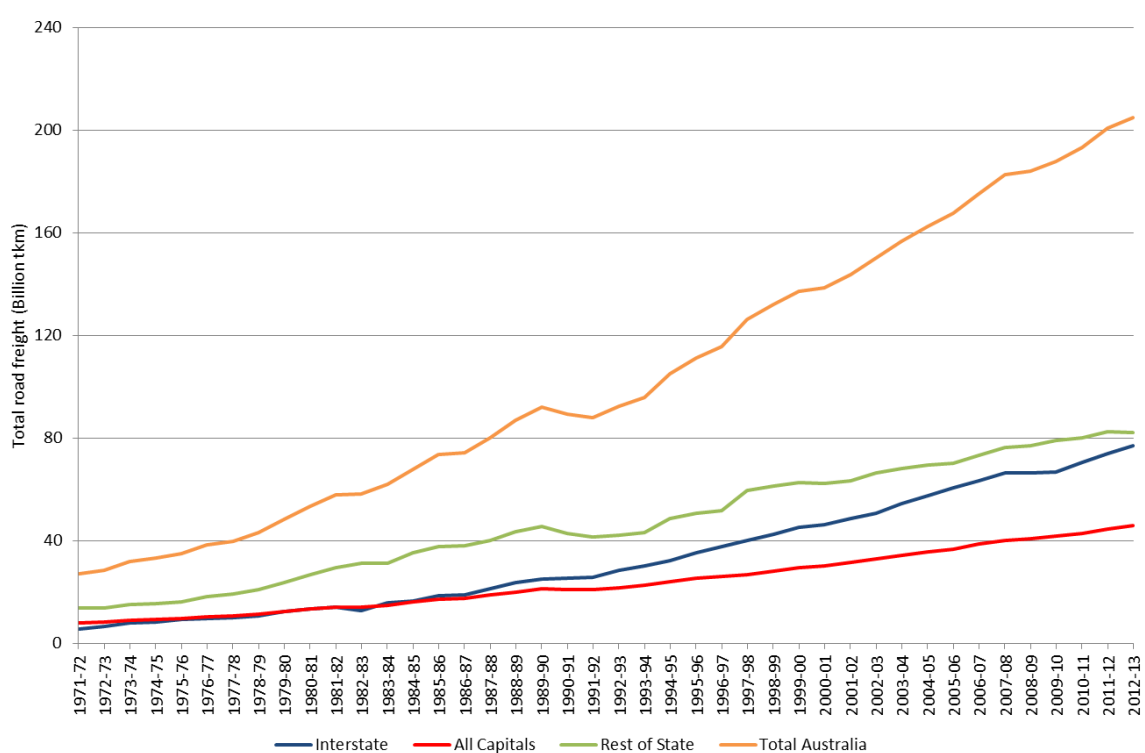
Figure 2.1 Road freight estimates by interstate, capital cities and rest of state, Australia, 1971-72 to 2012-13
